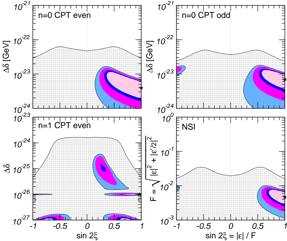
Figure 23: Allowed regions for the NP parameters for a future atmospheric neutrino experiment with 20 SK exposure and observed rates corresponding to the present SK data. The filled contours show the allowed region at 90%, 95%, 99% and 3\sigma CL. The hatched area is the presently excluded region at 3\sigma .
