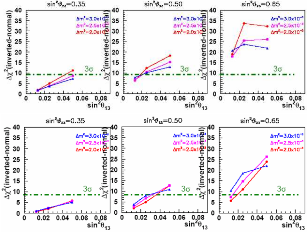
Figure 27: Statistical significance for measuring the sign of \Delta m^2_{23} for an exposure of 1.8 Mton yrs if the true hierarchy turns out to be normal (upper plots) or inverted (lower plots), for different values of |\Delta m^2_{23}| and \sin^2 \theta_{23} , as a function of \sin^2 \theta_{13} (same as in Fig. 26). Figure taken from Ref. [100].
