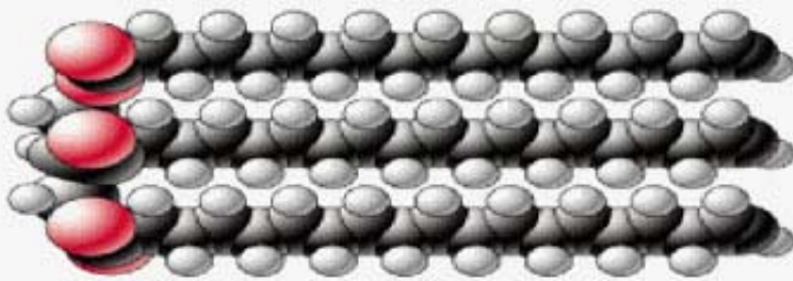
Tristearate
