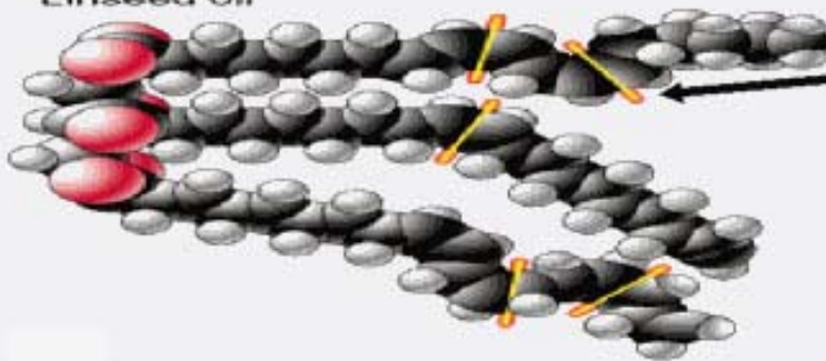
Linseed oil
