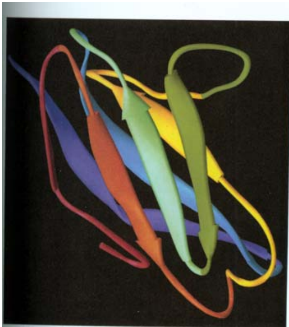
Immunoglobulin Folding (compare to \alpha -helix)
