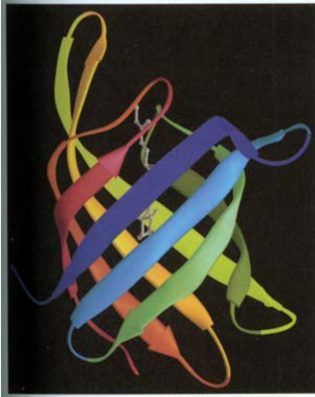
\beta -Barrel folding
